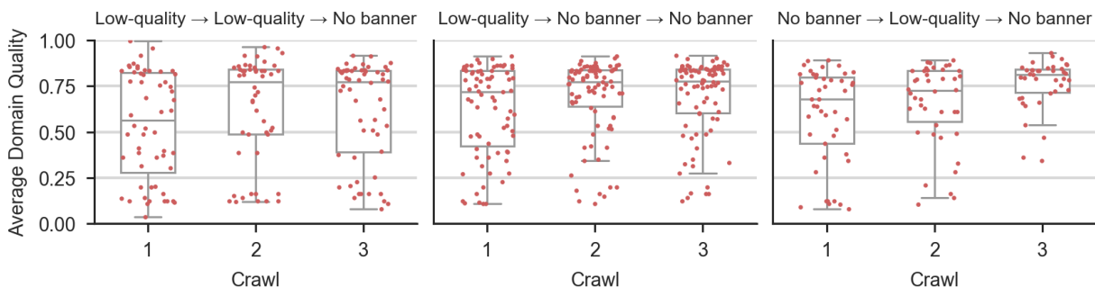
Figure 3: Many of the queries that received a low-quality banner in either (or both) of the first two crawls, continued to produce low-quality SERPs in the third crawl without a banner. Here we present the domain quality score distributions for the top three banner histories, which account for 85.9% of all banner histories that include a low-quality banner.
