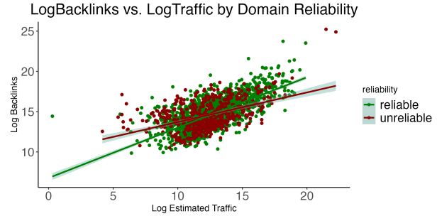
(b) Log backlinks vs log estimated traffic for labeled reliable and unreliable domains.
