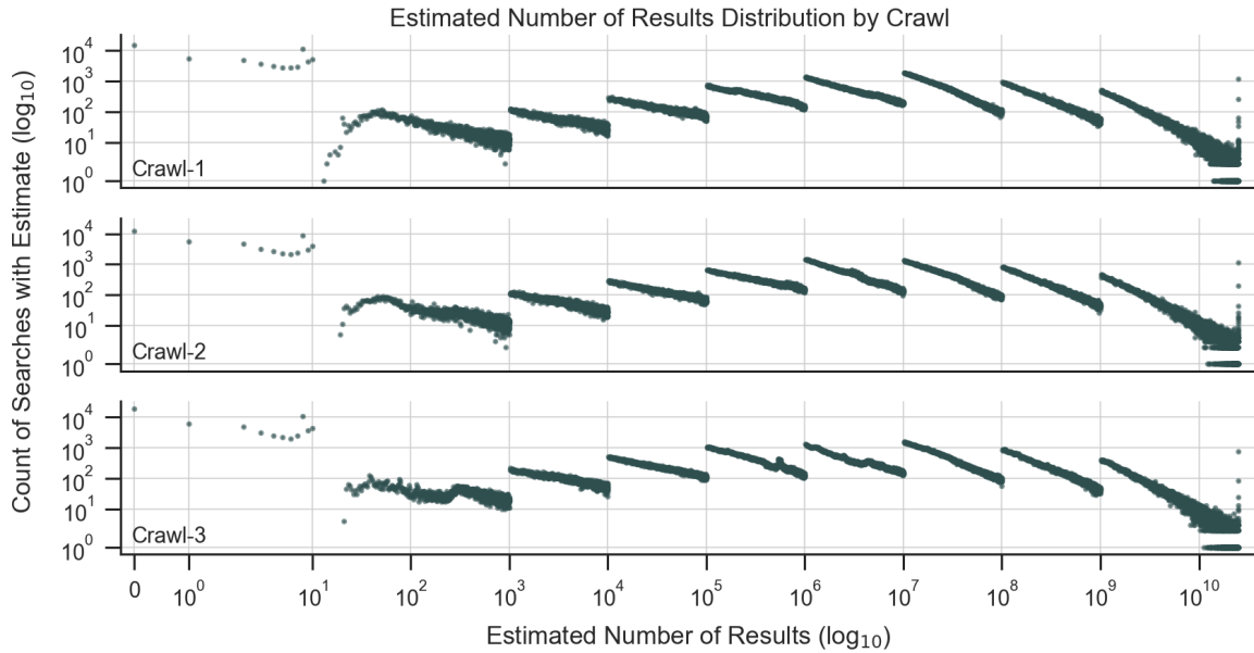
Figure 10: The estimated number of search results available for a given query—provided by Google in each SERP—follows a mixture distribution consisting of nine distinct distributions (e.g., 0 to 10 and 11 to 1000), suggesting different mechanisms for estimating the number of results within each band. The median number of estimated results was 4.6M in crawl-1, 3.3M in crawl-2, 1.9M in crawl-3, and 2.6M in crawl-4. Means ranged from 281M (crawl-1) to 204M (crawl-3) and standard deviations ranged from 1.4B (crawl-1) to 1B (crawl-4). Our data suggests a ceiling on Google’s estimates, and the max value we observed in any crawl was 25.27B.
