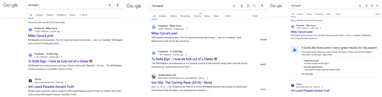
Figure 14: Search results for the query vrii lizard without (left screenshot) and with quotation marks (right two screenshots). All SERPs contain a similar set of URLs. The quoted version received a banner in one instance, but not in second screenshot taken a day later.
