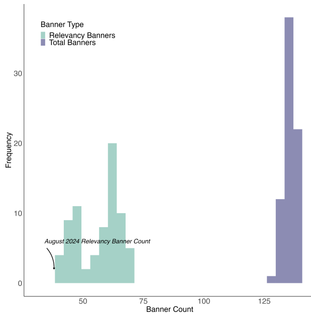
Figure 15: Quality banners do not appear to have been subsumed by low-relevance banners. We display histograms of the distributions of the counts of low-relevance banners over 73 time-steps (teal) and the distribution of total banners (i.e., low-relevance + low-quality) (purple). In August 2024, the count of low-relevance banners we observed was lower than we observed across any of the 73 June 2024 time-steps.
