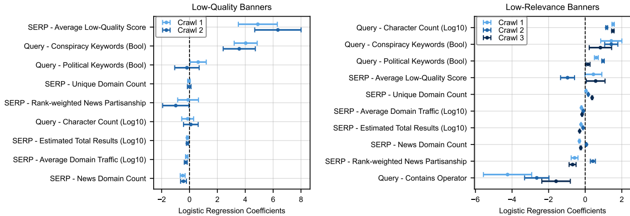
Figure 2: Across crawls, having low-quality domains in the SERP was the feature most associated with the presence of low-quality banners (left), while the length of a search query was the feature most associated with low-relevance banners (right). For both banner types, the use of conspiracy-related keywords in the search query was consistently the second largest positive association. In contrast, Google’s estimated total number of results, average domain traffic, and the number of news domains on a SERP all had a consistent negative association with the presence of either banner type. The use of an advanced operator in a search query had a consistent strong negative association with low-relevance banners, but queries containing such operators never produced a low-quality banner. Detailed regression tables are available in Appendix C.
