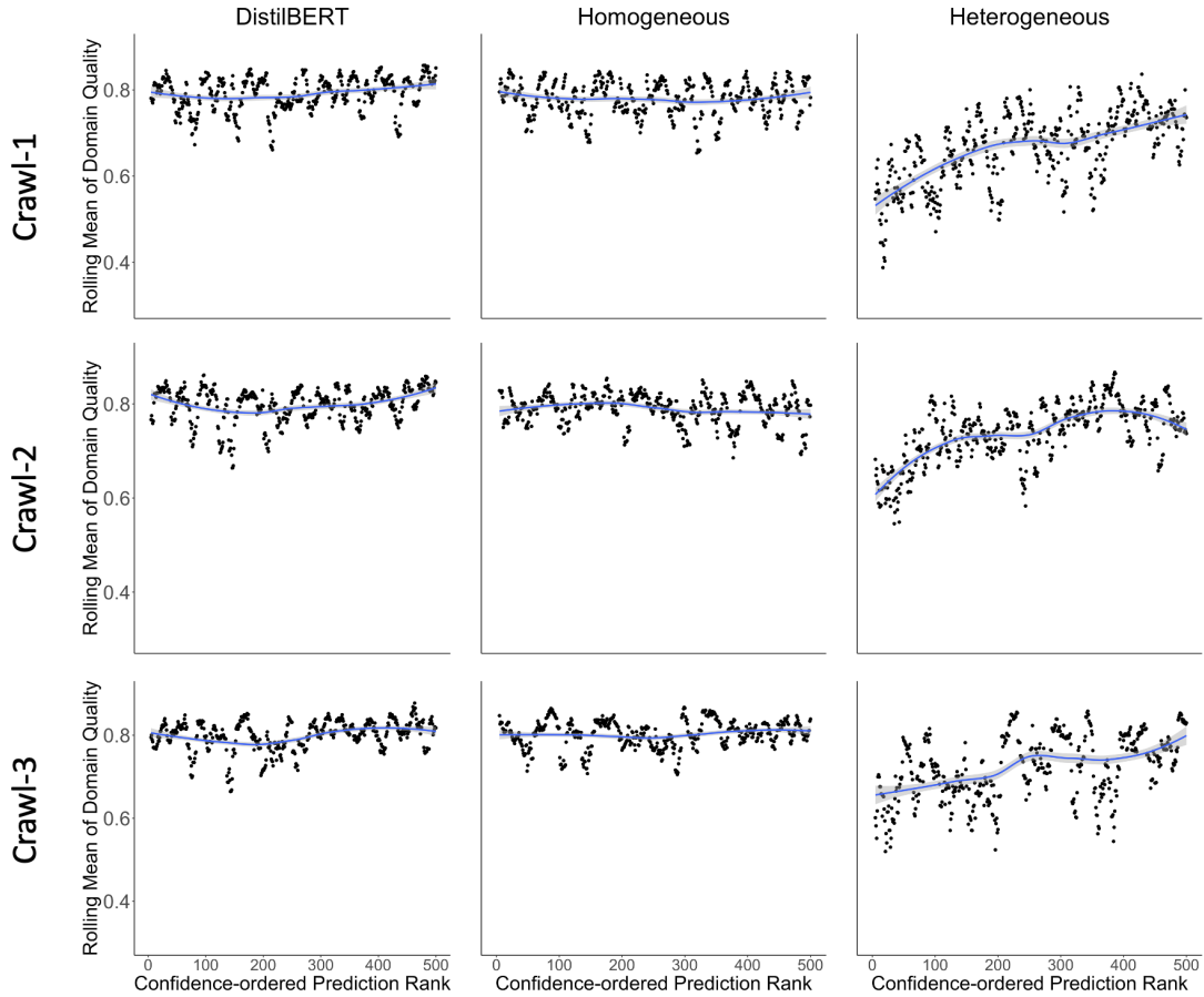
Figure 6: Heterogeneous GNNs best identify SERPs associated with unreliable domains. Each graph displays the rolling mean (window size of 10) of Domain Quality Scores over the 500 highest-confidence model predictions (lower scores indicate less reliable websites). With models trained on Crawl-1, we evaluated quality banner predictions for Crawl-1 (top), Crawl-2 (middle), and Crawl-3 (bottom).
