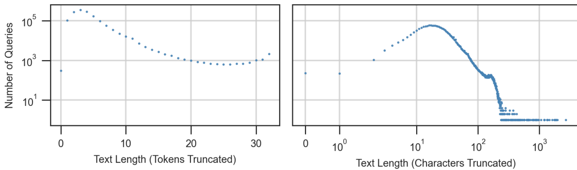
(b) Truncated search query length distribution.
