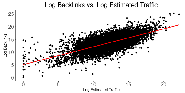
(a) Log backlinks vs log estimated traffic over all conspiratorial or political domains that ranked for at least 10 queries.
